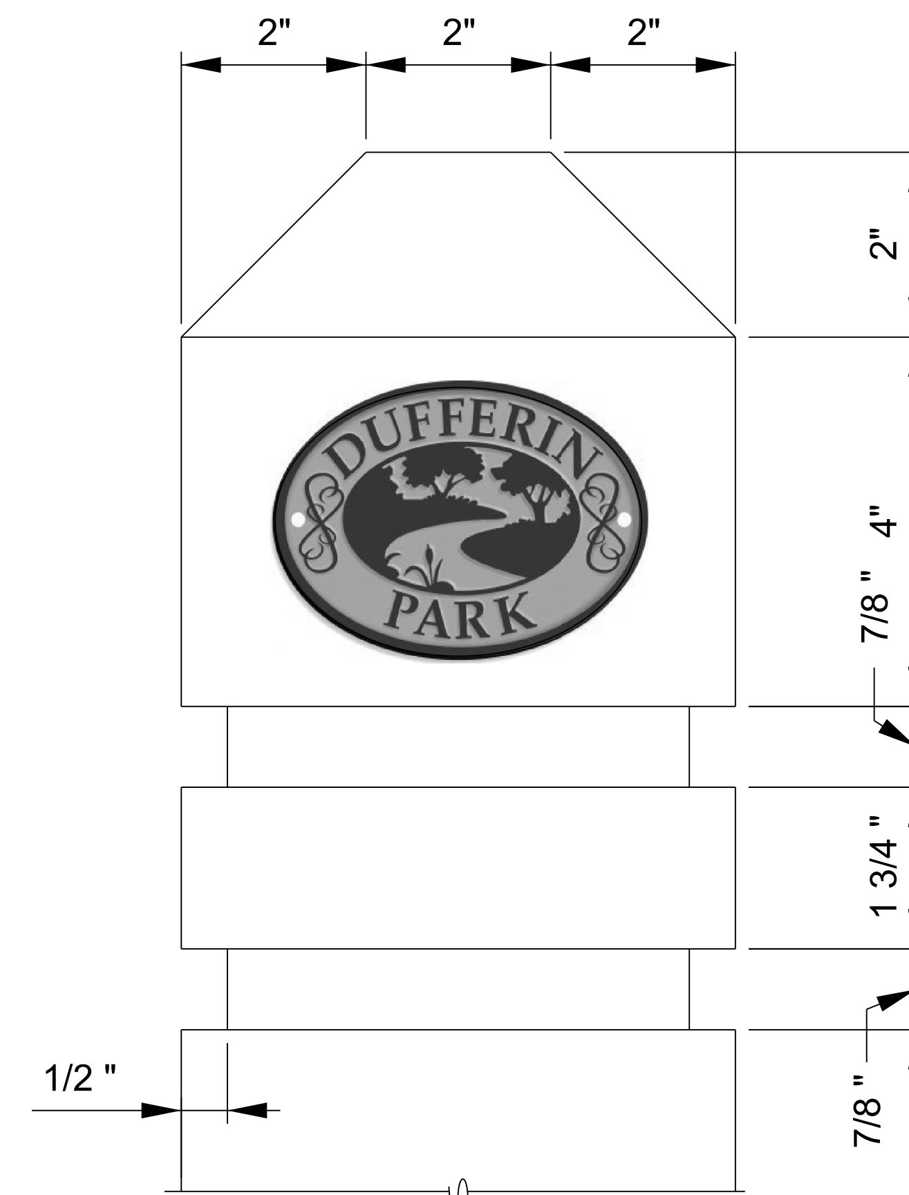
DETAIL A
