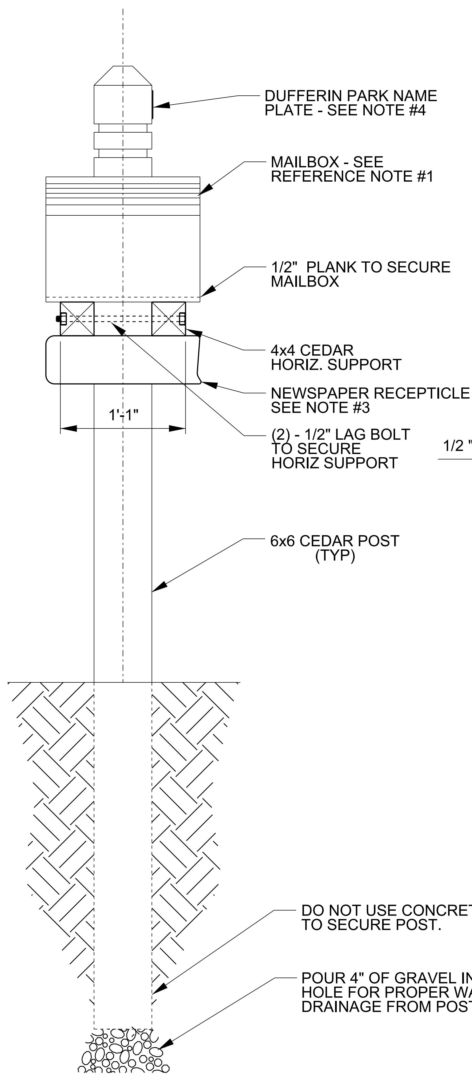
SIDE ELEVATION
