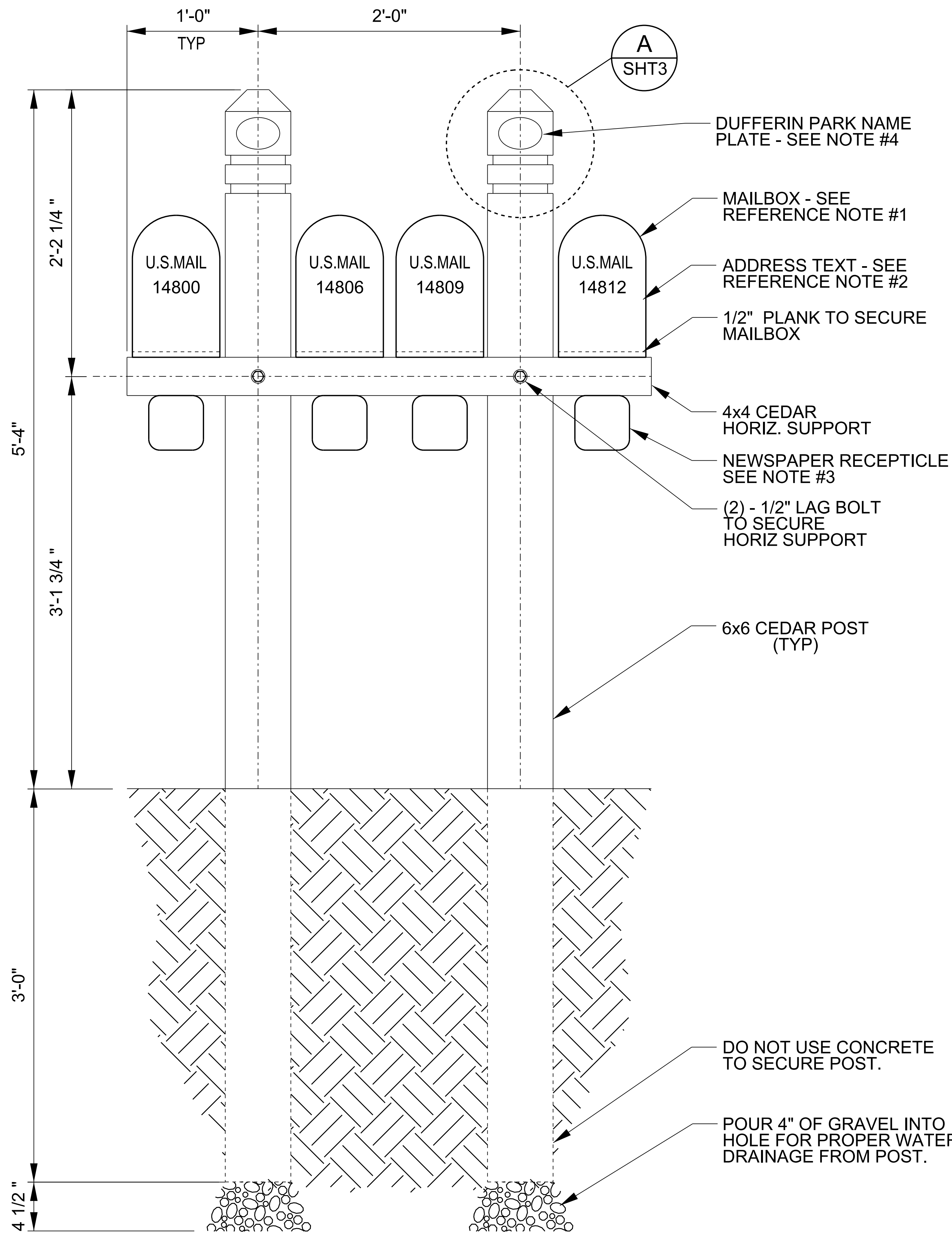
FRONT ELEVATION
