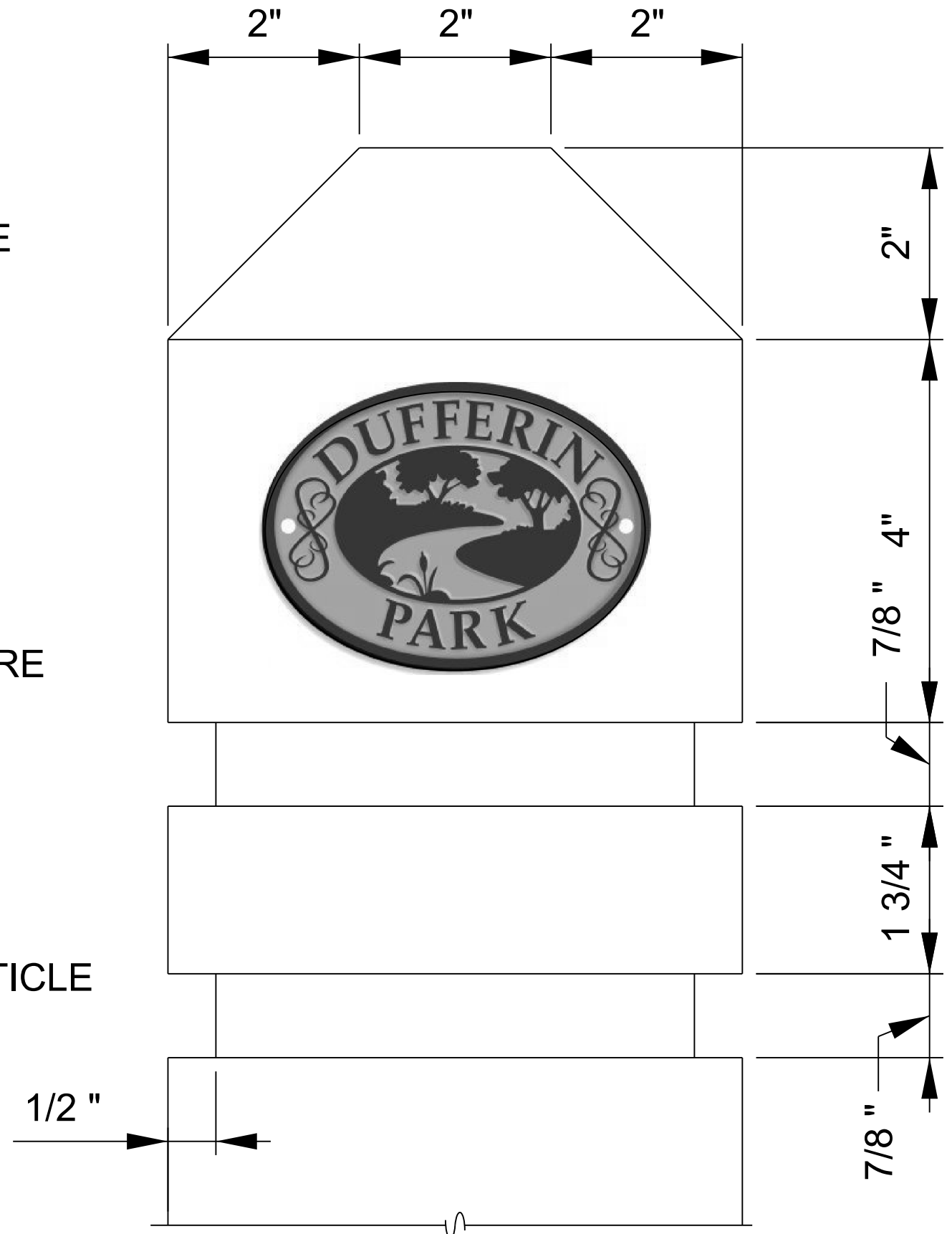
DETAIL A
